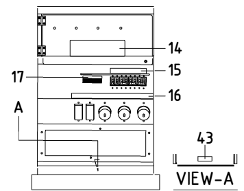
TERMINAL PLATE
